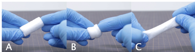
Figure 11. Due to its elasticity, our proposed sponge sensor can achieve both contraction and expansion, in contrast to prior methods.
