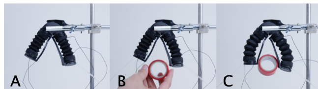
Figure 23. By using the tripod connector, three MorphIO modules can be used as a soft gripper.
