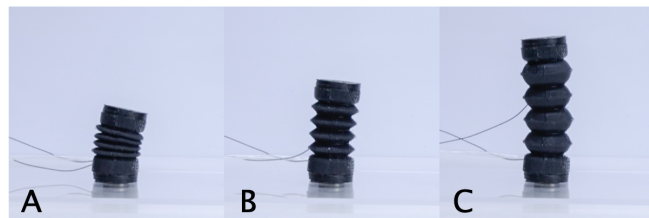
Figure 5. The contraction, neutral, and expanded states of the MorphIO unit. It can contract and expand up to 78% and 138% respectively.
