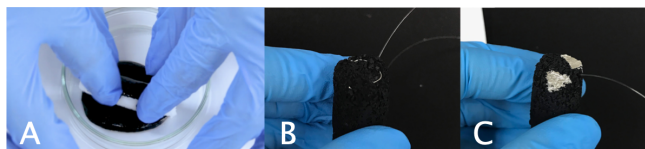
Figure 13. Impregnation of elastic sponge into conductive ink (A). Bonding the lead wire with the conductive sponge to make electrodes (B-C).
