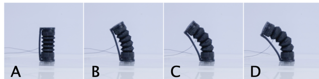
Figure 17. The technical evaluation of the bending capability.
