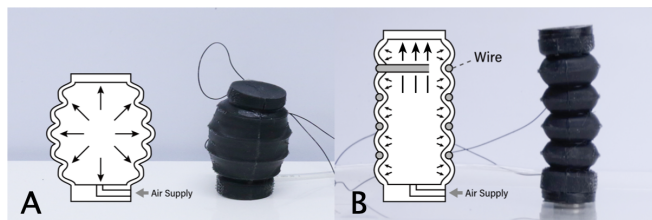
Figure 15. We wrap the bellows with a wire to ensure that the air pressure can only inflate in the vertical direction. Before using the wire (A). After using the wire (B).
