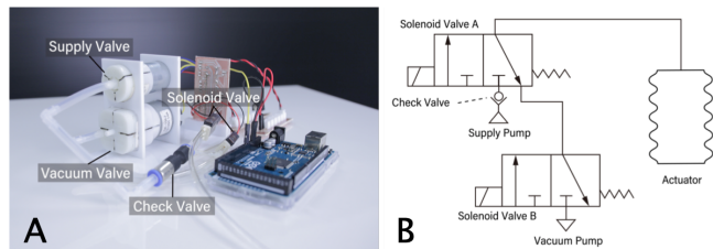
Figure 18. The pneumatic control circuit, consisting of two air pumps and two solenoid valves for supplying and vacuuming air (A). A schematic of the pneumatic control circuit (B).
