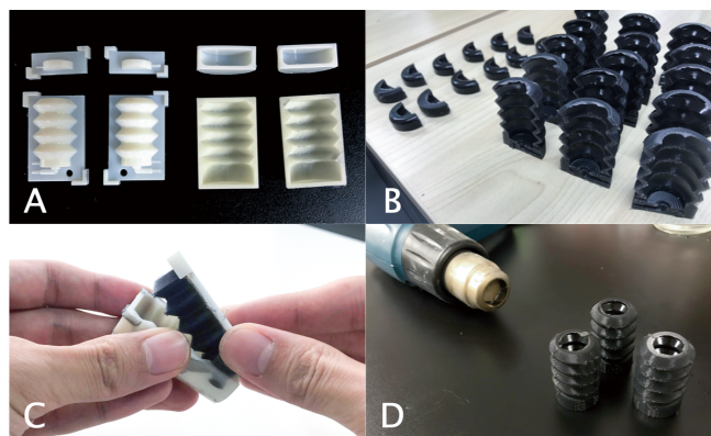
Figure 16. The fabrication process of the bellows pneumatic actuator. We embed the conductive sponge sensor into the internal air chamber of the bellows.
