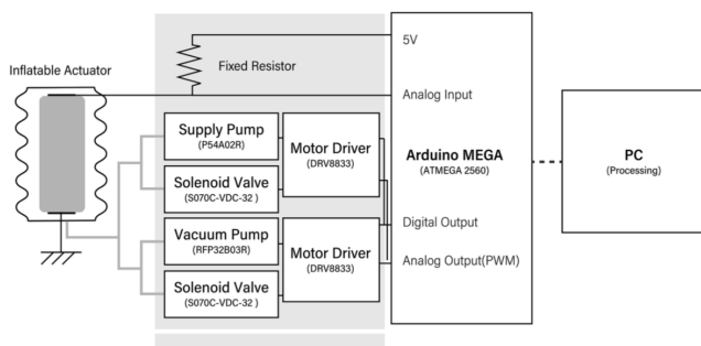
Figure 19. MorphIO's system design.
