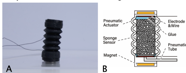
Figure 4. The MorphIO unit (A). Each unit consists of a bellows pneumatic actuator containing a conductive elastic sponge sensor (B).
