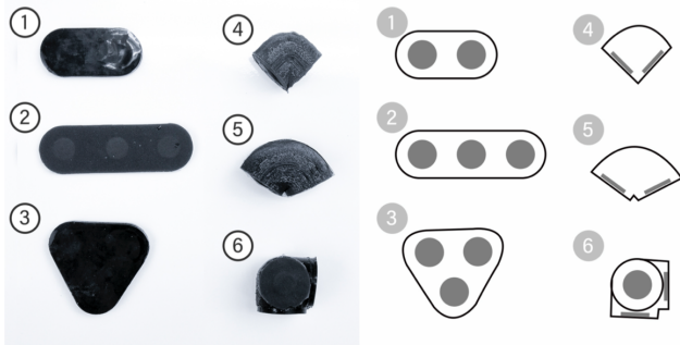
Figure 7. We designed and prototyped six different types connectors to allow for the easy construction of different topologies.
